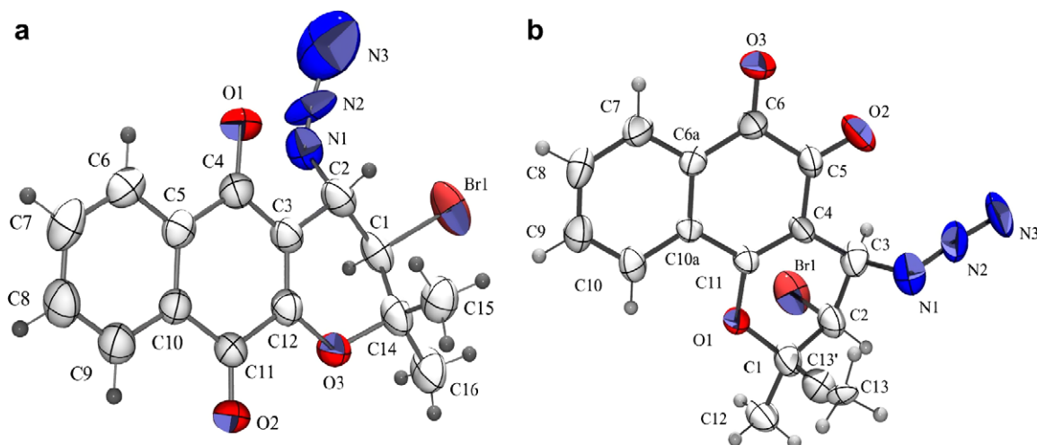
Figure 1. ORTEP3 projection of the compounds (a): 16 and (b): 17 , showing the atom numbering and 50% probability displacement ellipsoids.
